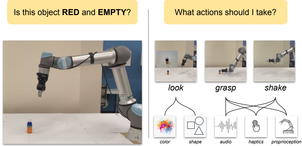
Figure 3.1: A robot is tasked with identifying if an object is RED and EMPTY . Given the various sensory modalities produced by exploratory behaviors, the robot must decide what behavior(s) to perform to gain maximum information.
